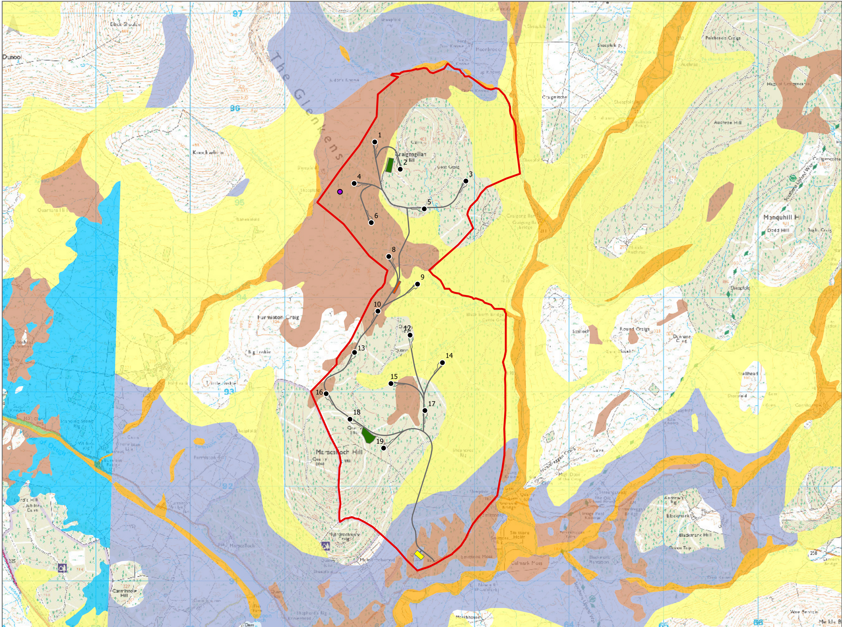
Figure 12.1: Superficial Soils
